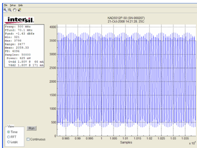
FIGURE 2. TIME-DOMAIN DISPLAY
